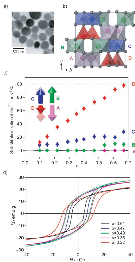
Figure 1. Crystal structures and magnetic properties of \epsilon - \text{Ga}_x\text{Fe}_{2-x}\text{O}_3 . a) TEM image for x = 0.61 . b) Crystal structure of x = 0.61 (space group: Pna2_1 ) projected from the [100] direction. Purple, green, and blue octahedra represent \{\text{FeO}_6\} units of the A, B, and C sites, respectively, while the red tetrahedra represent \{\text{FeO}_4\} units of the D site. c) The x dependence on the degree of \text{Ga}^{3+} substitution at the A (purple), B (green), C (blue), and D sites (red); the inset is a schematic diagram of the magnetic ordering of sublattice magnetization on A–D sites. d) Magnetization vs. external magnetic field plots for x = 0.22, 0.35, 0.40, 0.47 , and 0.61 at 300 K.
